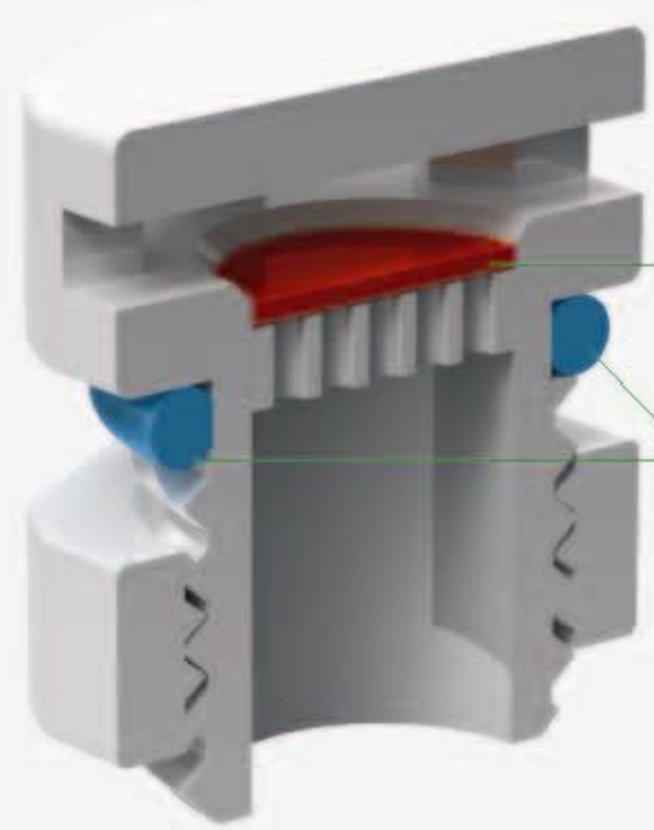
e-PTFE Breathable membrane Waterproof rubber ring
